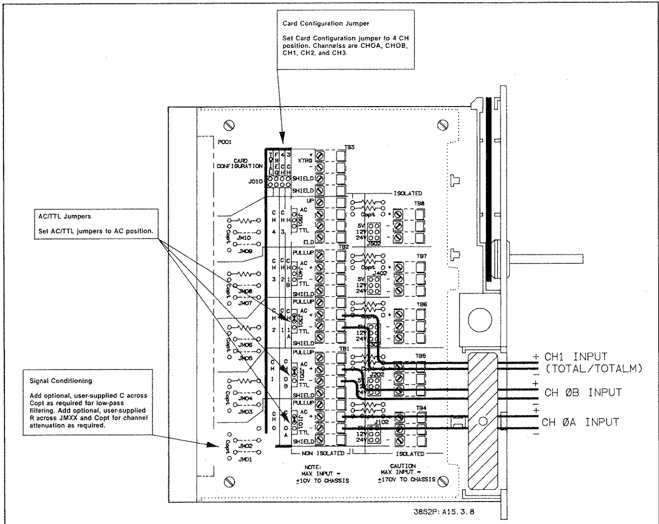
Figure 3-8. Example: Non Isolated Channels - Field Wiring
